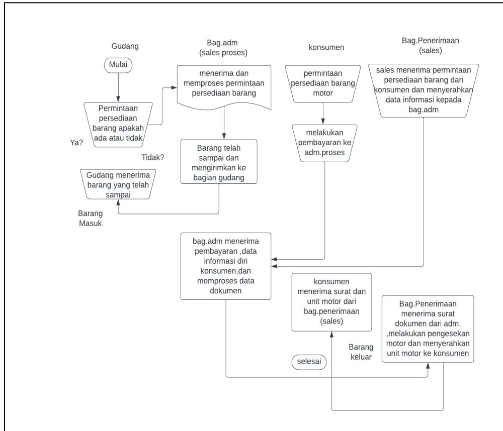
Gambar 3.2 Flowchart Versi Peneliti
